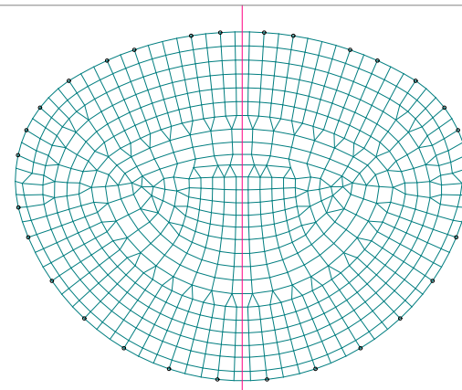
INNER CHORD
