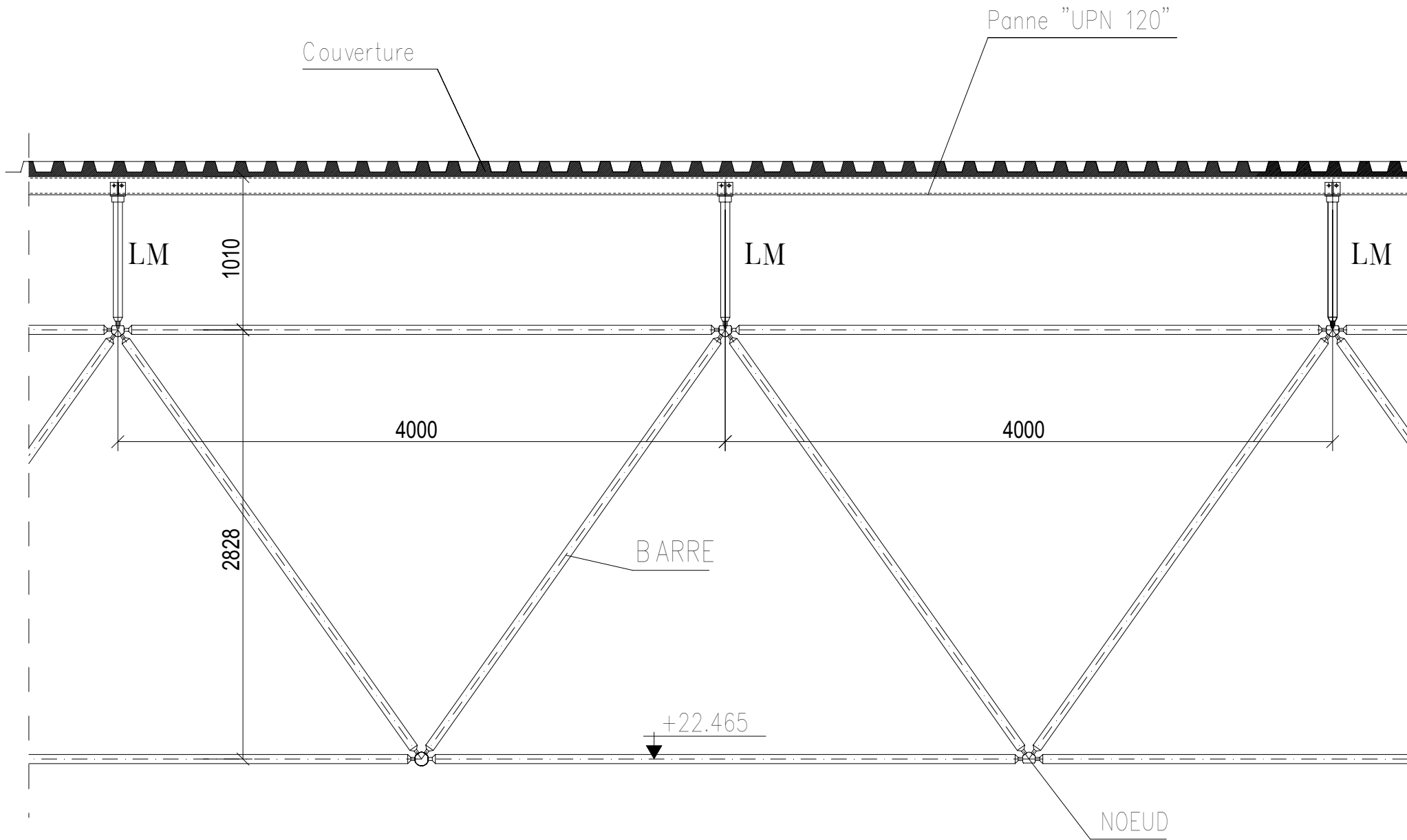
DETAIL F
