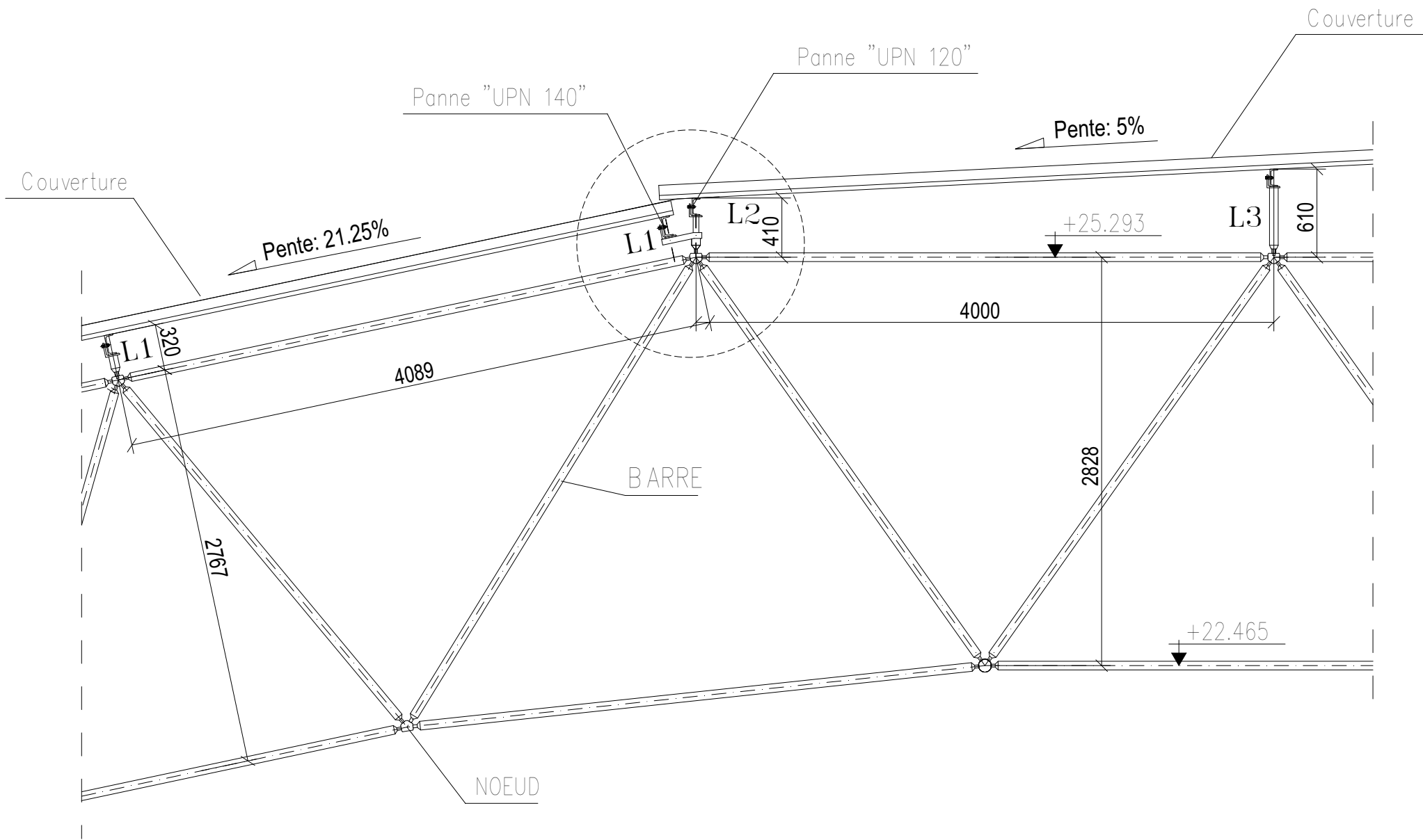
DETAIL B
