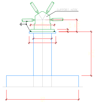
DETAIL B (P2)
